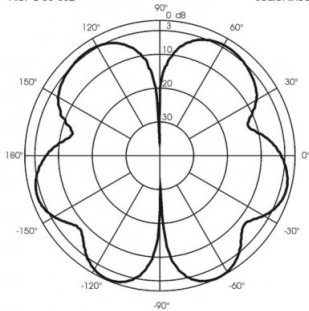
TYPICAL RADIATION PATTERN in E-plane at 437 MHz File: E-05-002 Scale: linear
